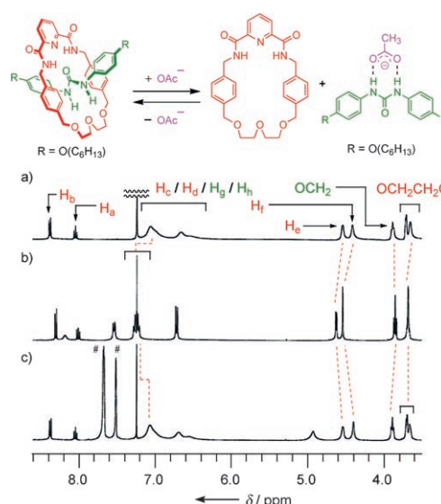
Figure 1. Partial ^1\text{H} NMR spectra (400 MHz, \text{CDCl}_3 , 298 K) of a) an equimolar mixture of 1 and 3 (10 mM), b) the mixture obtained after adding TBAA (2 equiv) to the solution in (a), and c) the mixture obtained after adding \text{NaBARF}_4 (2 equiv) to the solution in (b). #: Signals from \text{NaBARF}_4 .
